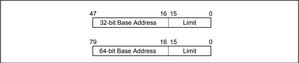
Figure 3-11. Pseudo-Descriptor Formats
