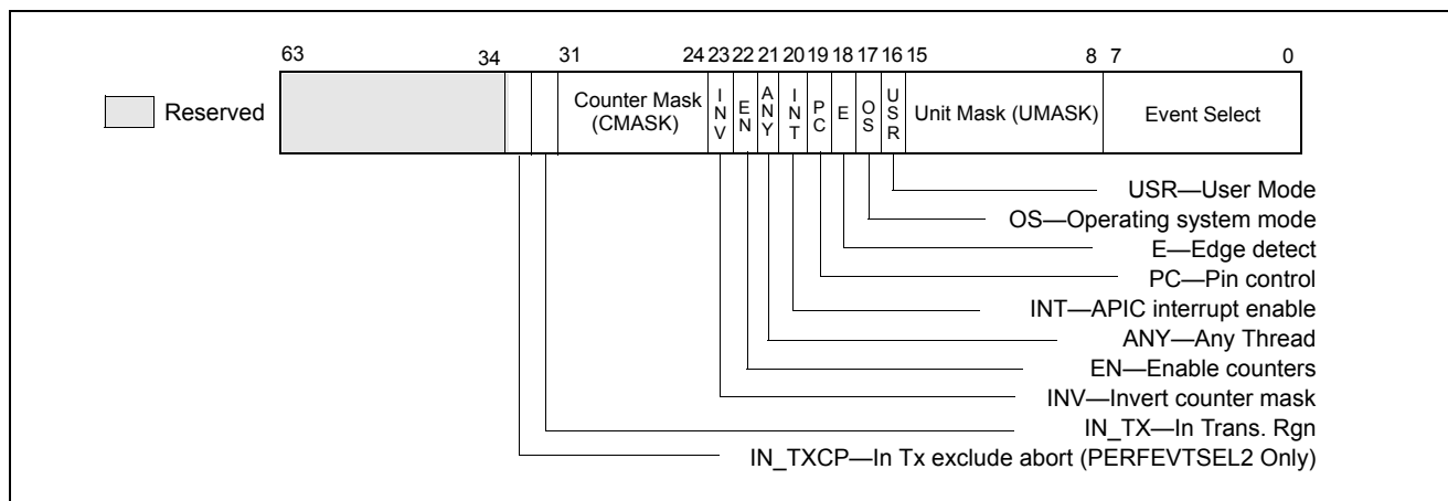
Figure 18-40. Layout of IA32_PERFVTSELx MSRs Supporting Intel TSX
