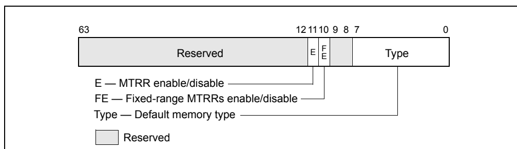
Figure 11-6. IA32_MTRR_DEF_TYPE MSR
