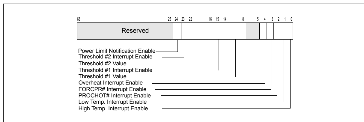
Figure 14-29. IA32_THERM_INTERRUPT Register
