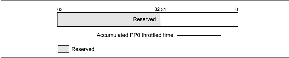
Figure 14-40. MSR_PP0_PERF_STATUS MSR
