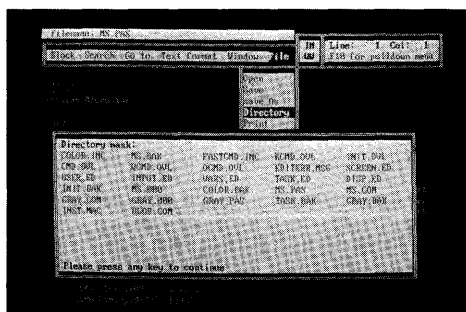
MicroStar's pull-down menus.
