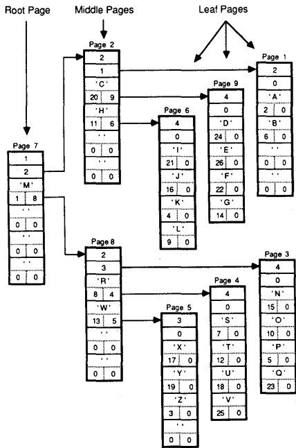
Figure B-6. Diagram of a B + tree of Order 2
