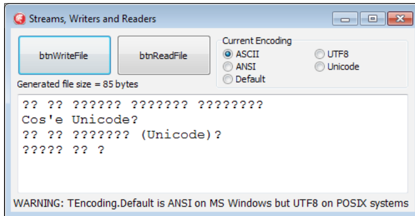
Garbage text written to the file using the wrong encoding. No one line of text is equal to the original one. It is necessary to know the encoding for the text before writing and reading it.
