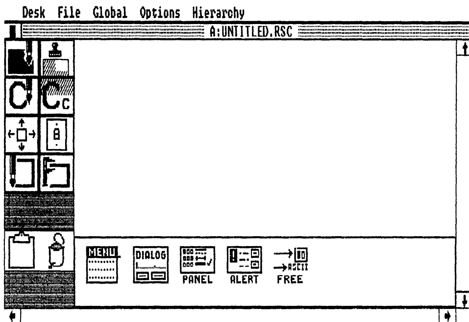
Fig. 7-2. The Resource Construction Set (RCS) develops the graphics for applications and desk accessories.
