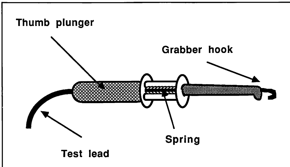
Figure 2-4 Grabber
